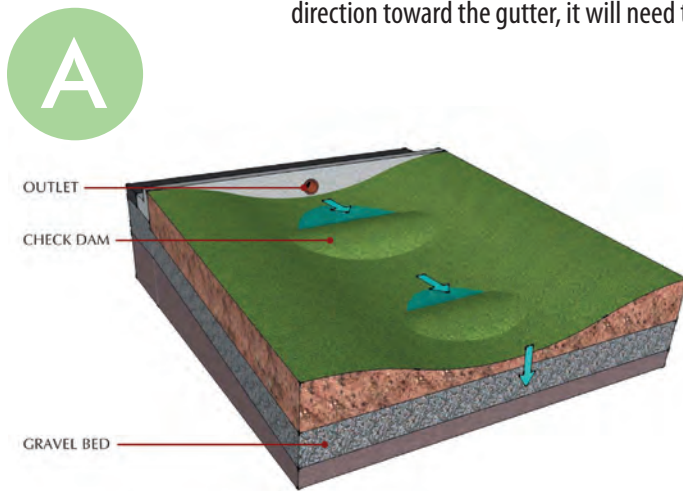
Diagram A: Drainage Swale
