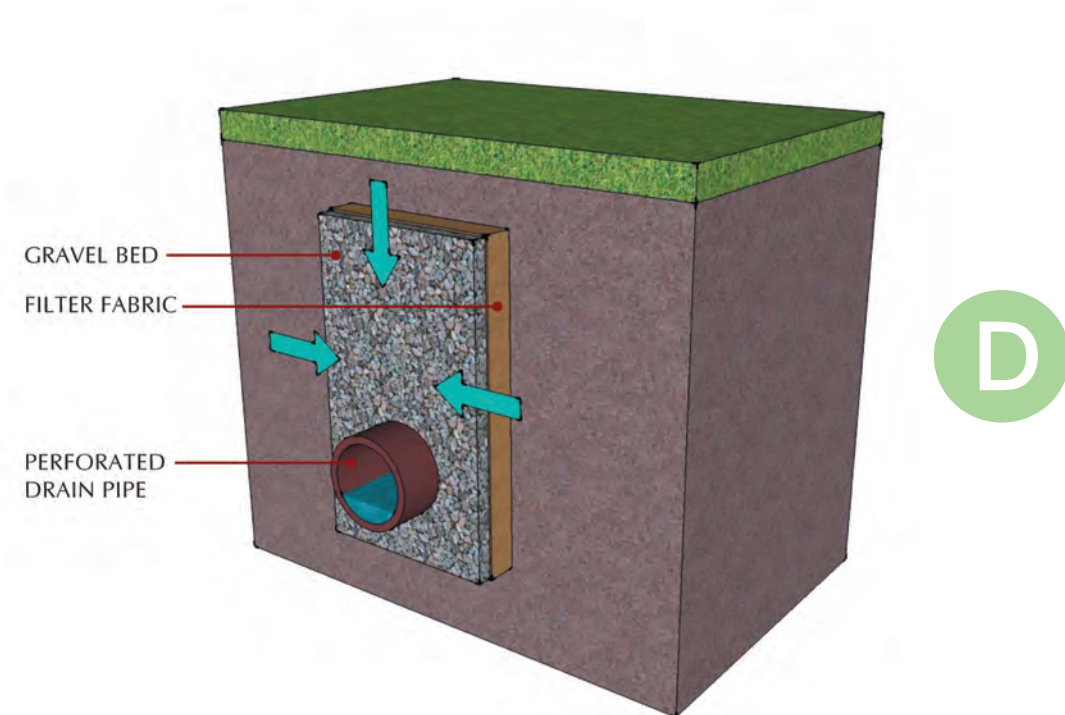
Diagram D: French Drains
