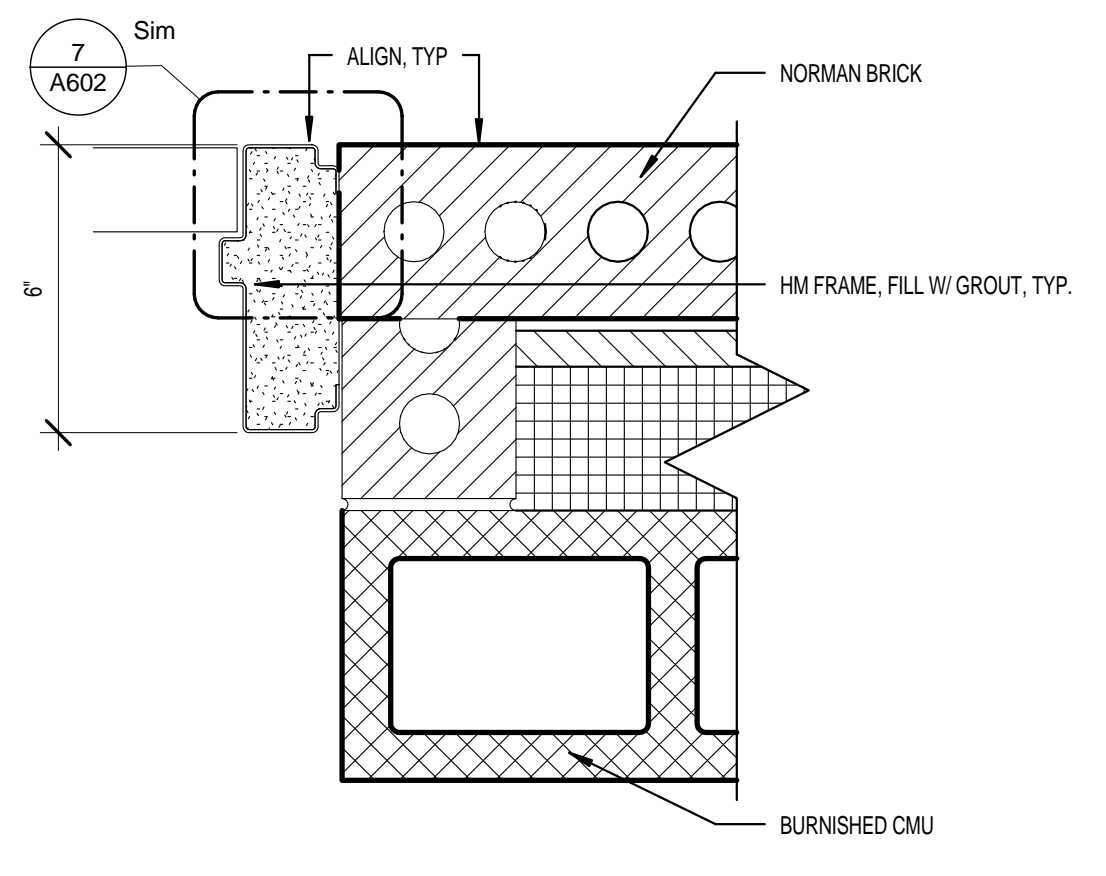
2 DR JAMB DETAIL - EXT. MASONRY OPENING
