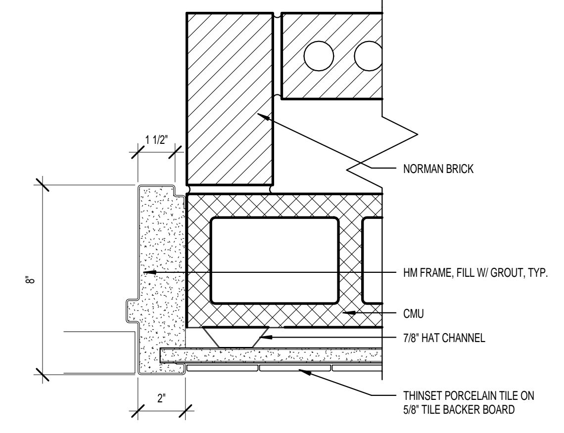
1a DR JAMB DETAIL - MASONRY @ TOILET RM
