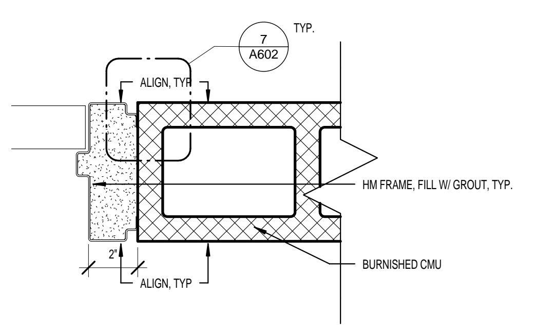
3 DR JAMB DETAIL - CMU OPENING
