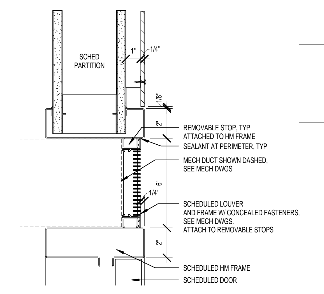
8a SECTION DETAIL - LINEAR DIFFUSER AT FRAME TYPE 5
