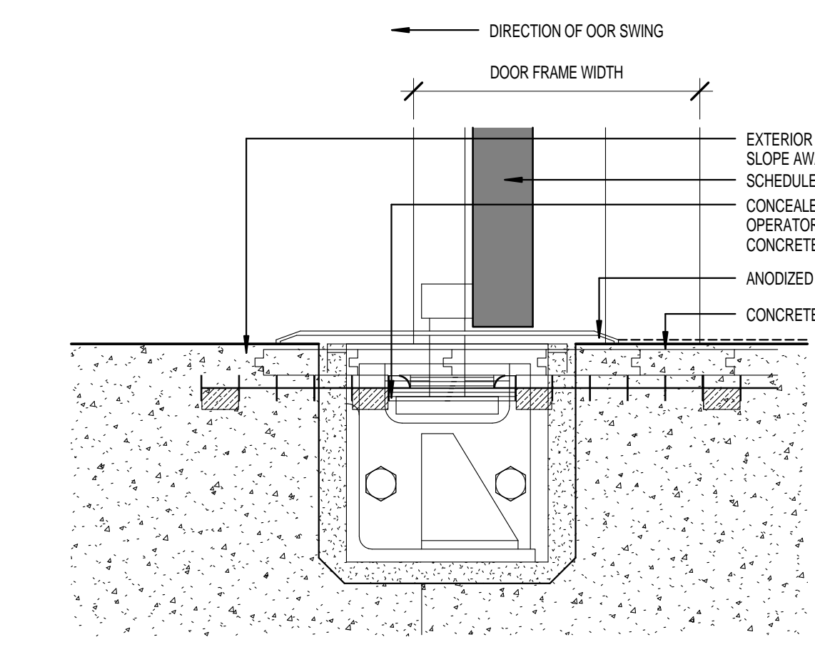
13 DR THRESHOLD DETAIL - EXTERIOR DOOR W/ CLOSER
