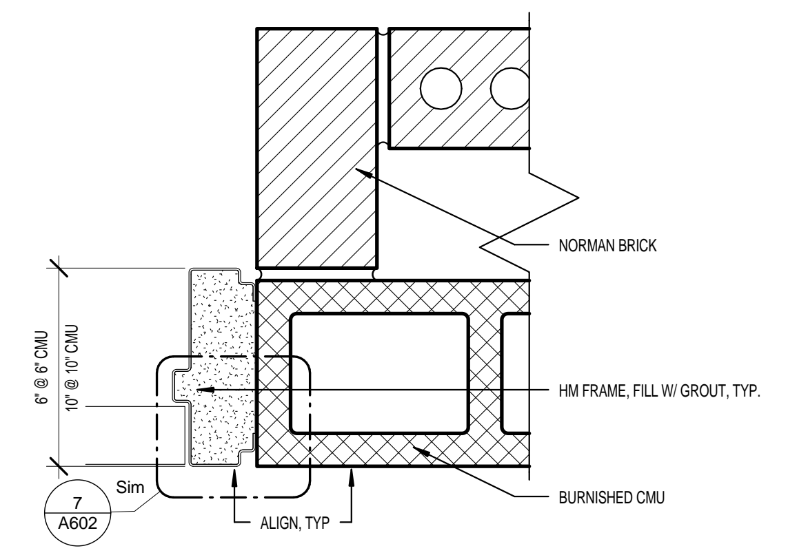
1 DR JAMB DETAIL - MASONRY OPENING
