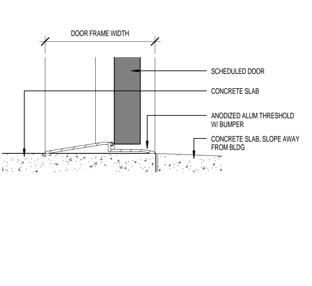
11 DR THRESHOLD DETAIL - EXTERIOR DOOR
