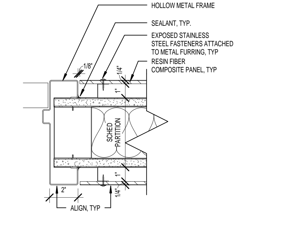
4 DR JAMB DETAIL - RESIN BD BOTH SIDES
