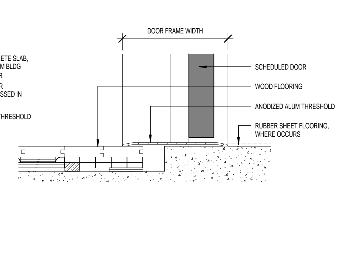
12 DR THRESHOLD DETAIL - WOOD FLOORING TO RUBBER/CONC.
