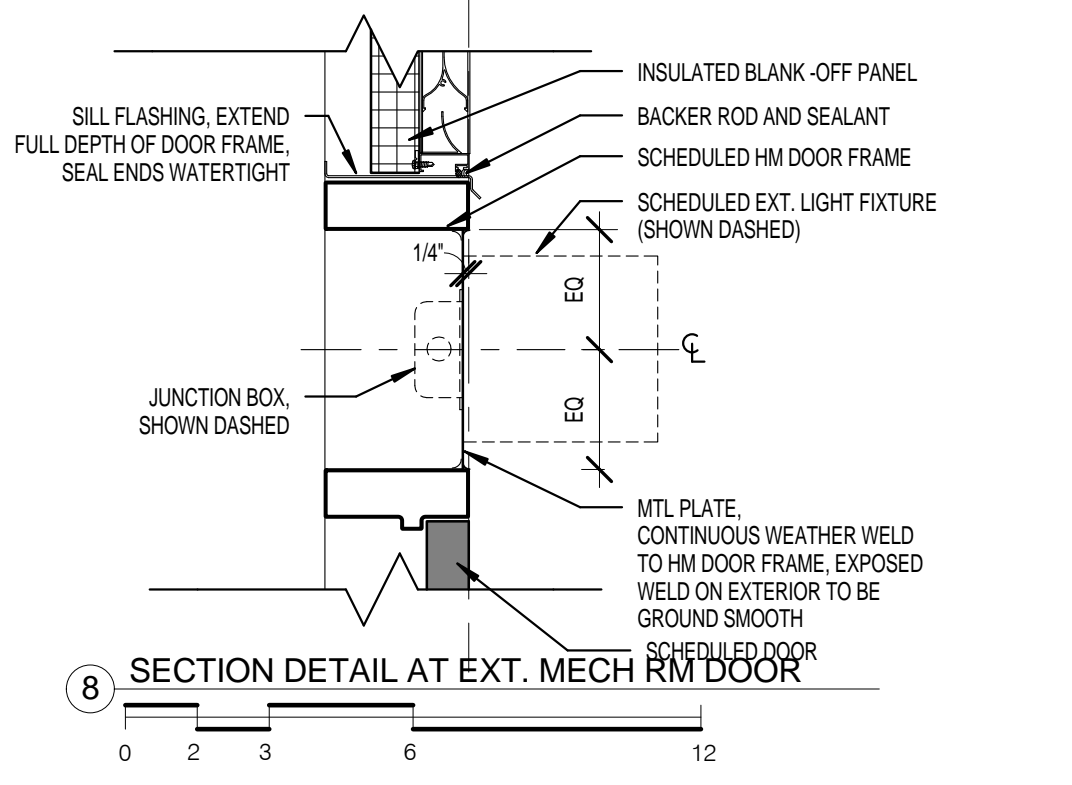
8 SECTION DETAIL AT EXT. MECH RM DOOR
