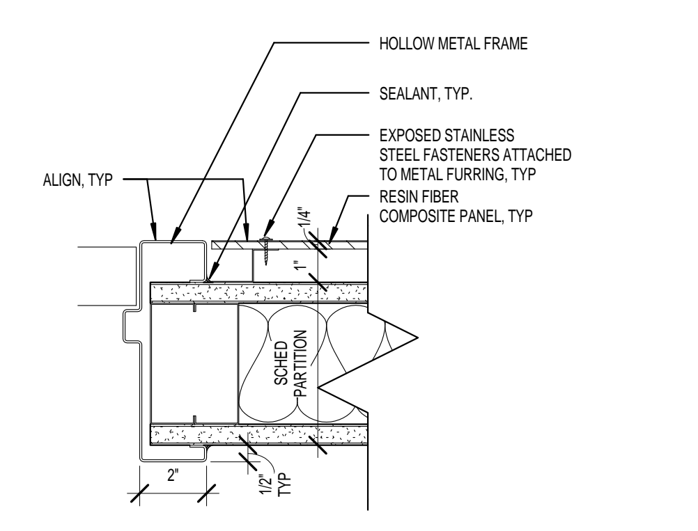
5 DR JAMB DETAIL - RESIN BD ONE SIDE
