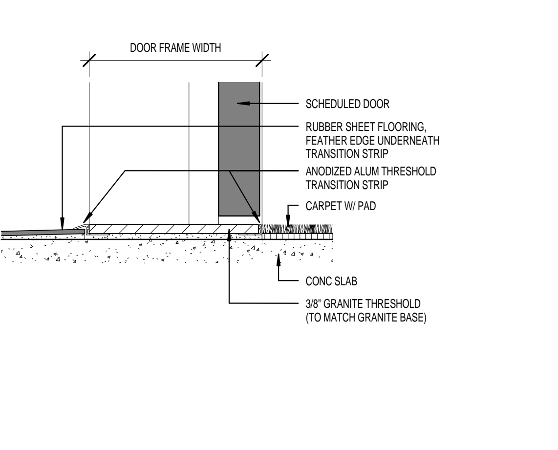
10 DR THRESHOLD DETAIL - RUBBER TO CARPET
