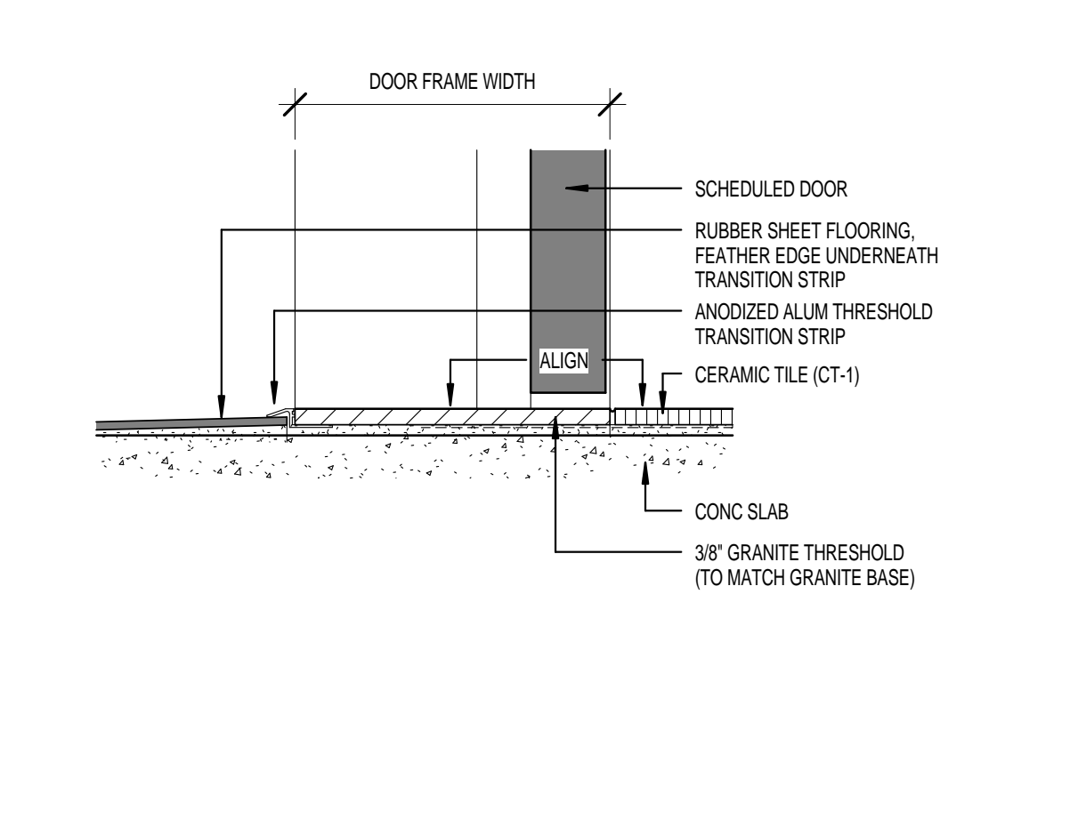
9 DR THRESHOLD DETAIL - RUBBER TO CERAMIC TILE
