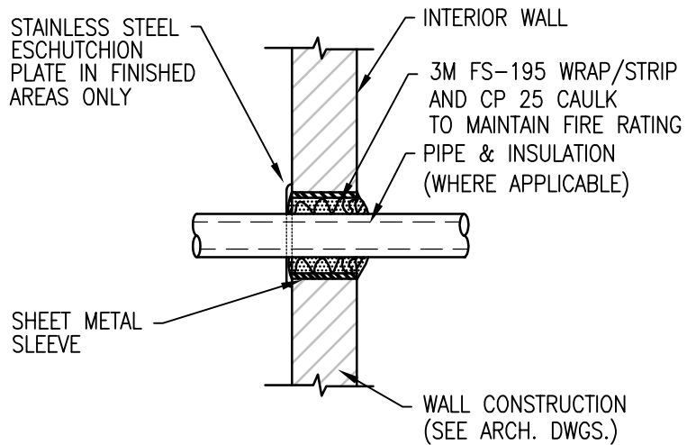
FIRE RATED WALL PENETRATION DETAIL
